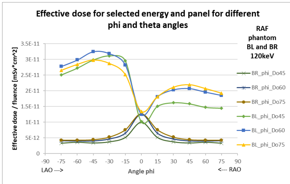
Figure 4: Effective dose per fluence conversion coefficients for photons of energy 120 keV for the Bottom left (BL) and Bottom right (BR) panels of the RAF phantom. The x-axis is representing different horizontal angles, and each vertical angle is represented by a different curve.
