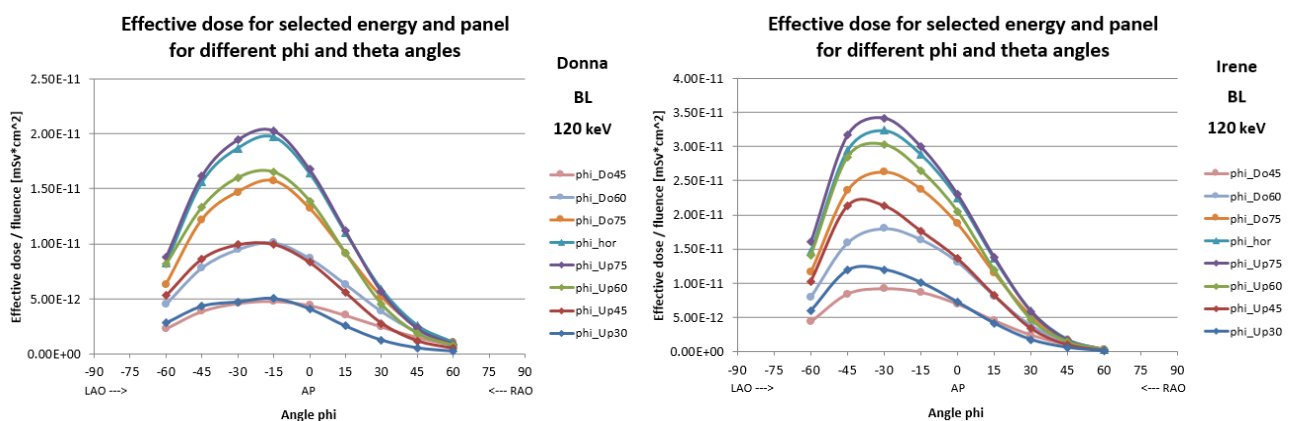
Figure 2: Effective dose per fluence conversion coefficients for photons of energy 120 keV for the Bottom left (BL) panels of Donna2018 (left) and Irene2018 (right). The x-axis is representing different horizontal angles, and each vertical angle is represented by a different curve.
