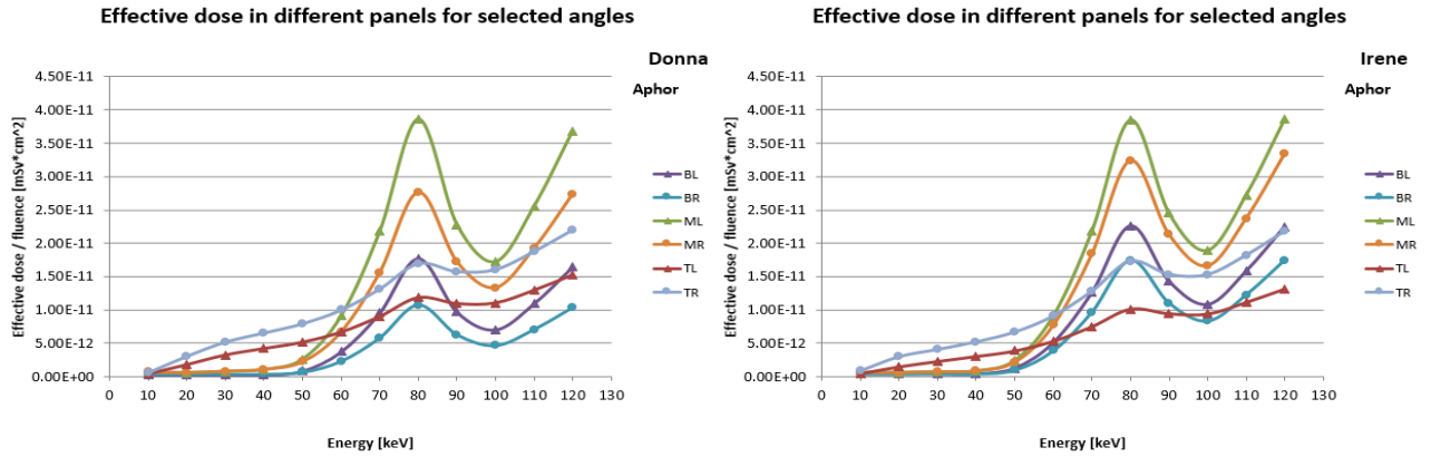
Figure 3: Effective dose per fluence conversion coefficients for AP horizontal radiation incidence for Donna2018 (left) and Irene2018 (right). The x-axis is representing photon energy, and each panel is represented by a different curve.
