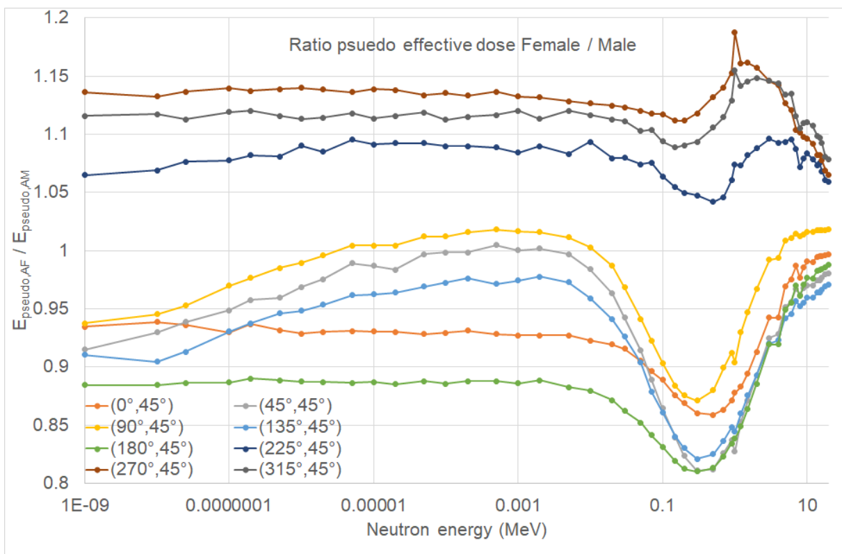
Figure 4: Ratio of the pseudo effective dose per fluence conversion coefficient for the Adult Female / Adult Male phantom for various neutron energies, and various horizontal angles (first in legend) and the vertical 45^\circ upwards (second in legend) direction.
